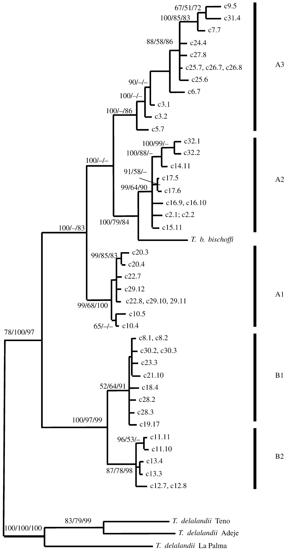
Figure 1. Bayesian phylogram of T. boettgeri mitochondrial (mt) haplotypes. Samples from Gran Canaria are marked with 'c', the following number gives the locality number, the number after the dot gives specimen number. Outgroups are T. delalandii from Teno, Adeje area and La Palma. Major clades are indicated by bars. Numbers on branches ( \geq 65 ) give Bayesian posterior probabilities and bootstrap values for ML and MP reconstruction, respectively.
