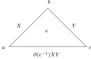
Figure 3: A \mathcal{G} -colouring of an ordered non-degenerate 2-simplex. Here X, Y \in G, e \in E and a < b < c are vertices of M . To this \mathcal{G} -colouring we associate the morphism XY \xrightarrow{e} \partial(e)^{-1}XY , in the category \mathcal{C}(\mathcal{G}) .
