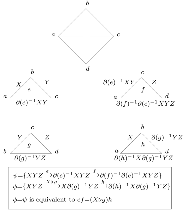
Figure 4: A \mathcal{G} -colouring of an ordered non-degenerate tetrahedron. Here a < b < c < d . Note that the compatibility condition ef = (X \triangleright g)h ensures that \partial(f)^{-1}\partial(e)^{-1}XYZ = \partial(h)^{-1}X\partial(g)^{-1}YZ .
