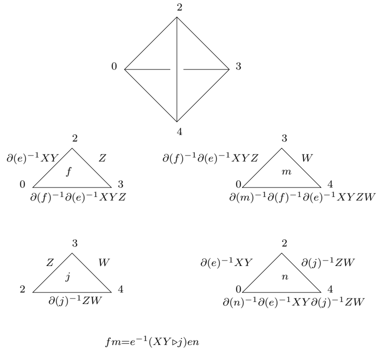
Figure 7: The most general \mathcal{G} -colouring of (01234): restriction to (0234).
