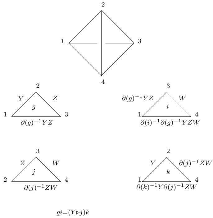
Figure 6: The most general \mathcal{G} -colouring of (01234): restriction to (1234).
